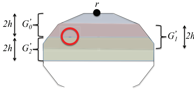
FIG. 3.2. A decomposition of a graph G' into overlapping 2h -outerplanar graphs according to a breadth-first search of G' that starts in an arbitrary vertex r . The shortest cycle is guaranteed to be completely contained within one of these 2h -outerplanar graphs, in this case in G'_1 .
